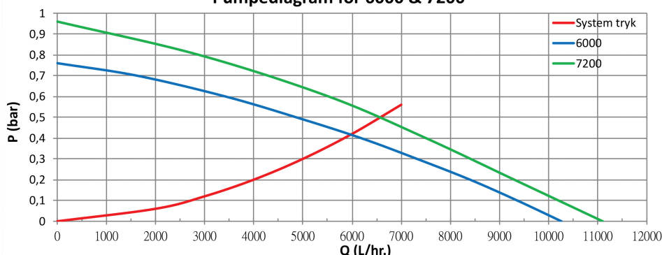
Pumpediagram for 6000 & 7200
